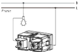
1-way switch
