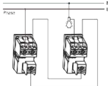
3/2-way switch
